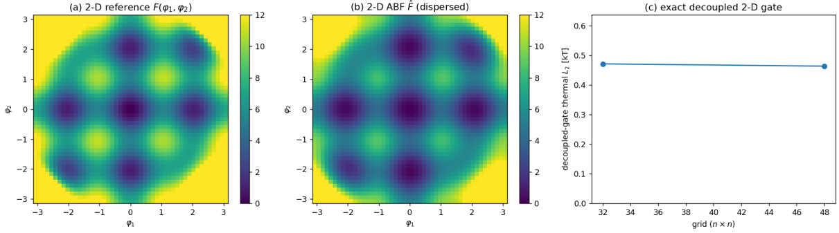
Figure 36: (a) the joint reference F(\varphi_1, \varphi_2) ; (b) a representative 2-D ABF reconstruction; (c) the exact decoupled gate L_2 versus grid resolution — flat, showing the residual is the mean-force estimator floor rather than a grid-discretisation error.
