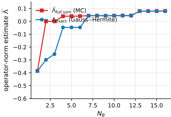
separable, \kappa = 5
