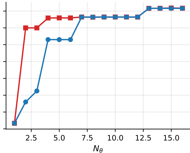
separable, \kappa = 100
