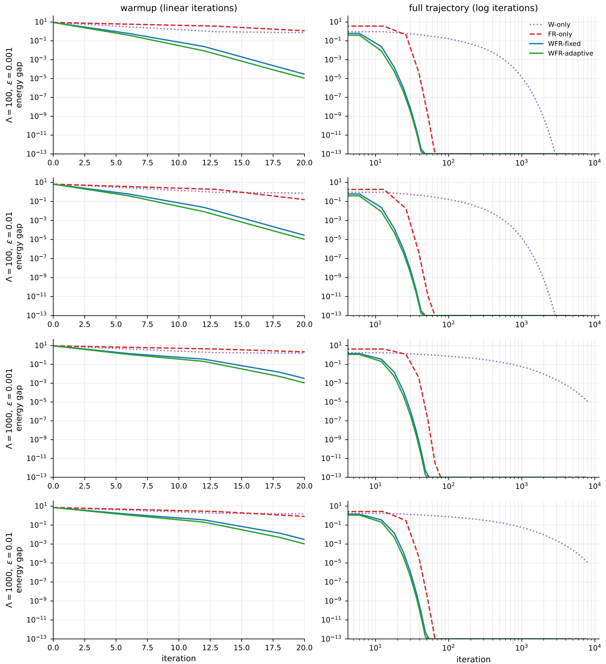
Gaussian posterior: WFR phase separation (gap vs iteration)
