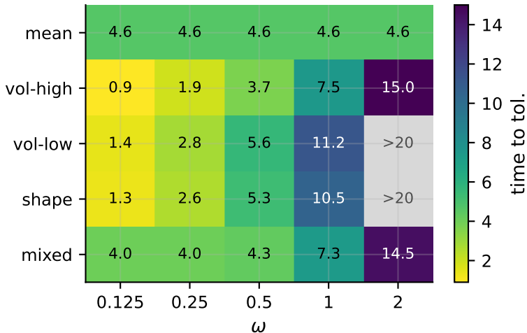
Gaussian, n = 5 : time to F/F_0 \leq 10^{-4} ( \tau = 0 )
