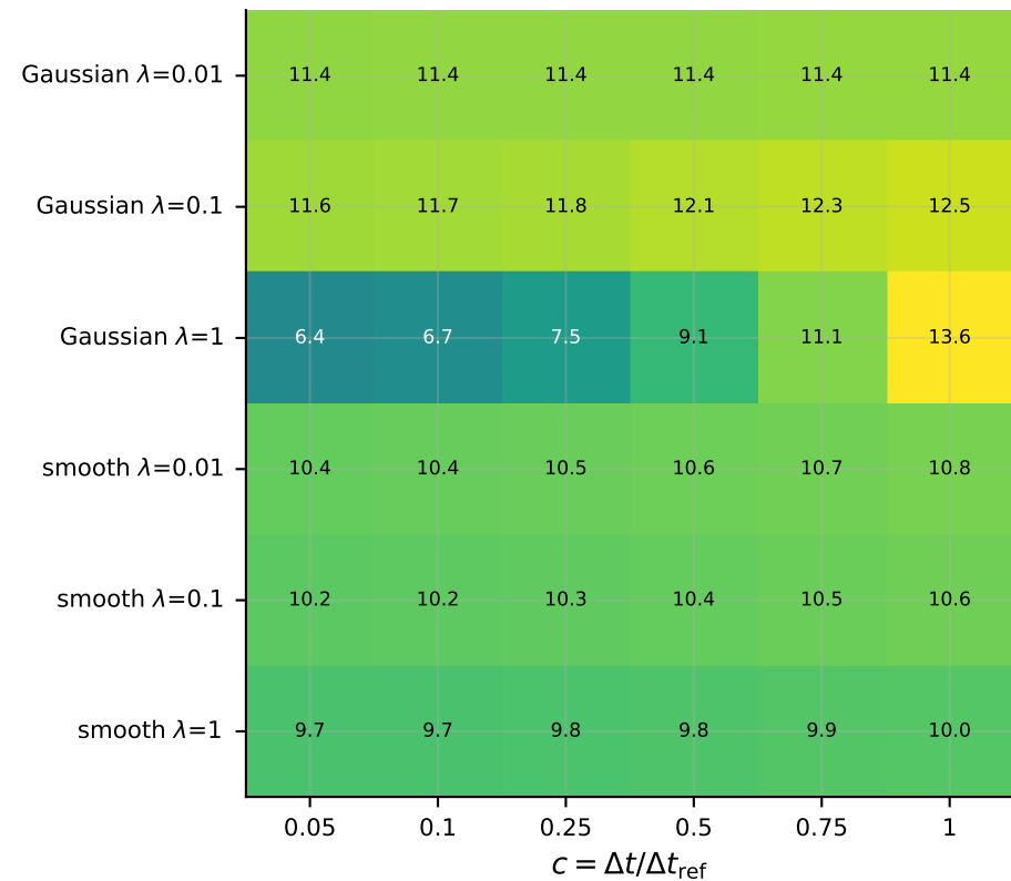
Riemannian
