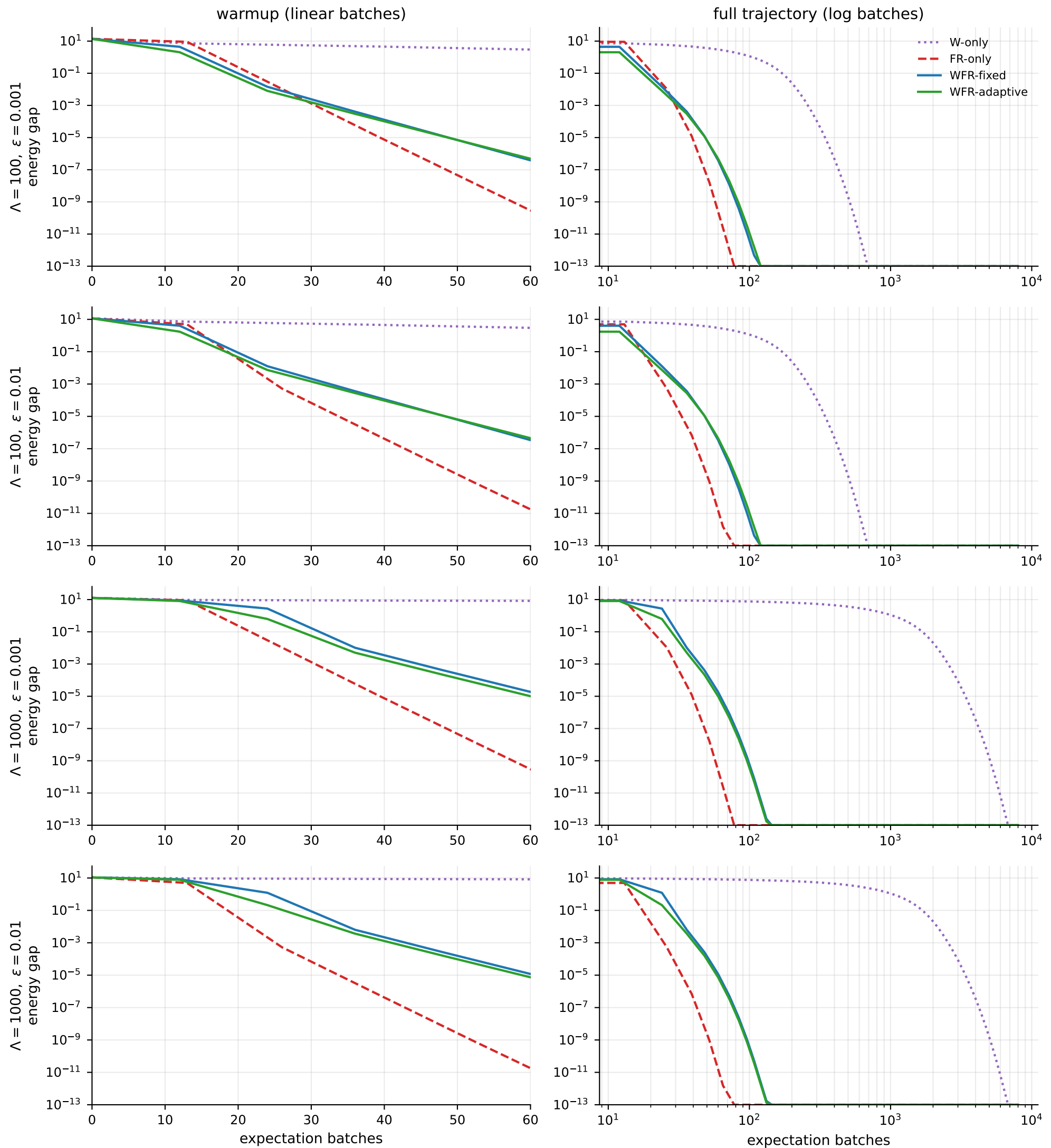
smooth log-cosh posterior: WFR phase separation (gap vs expectation-batch cost)
