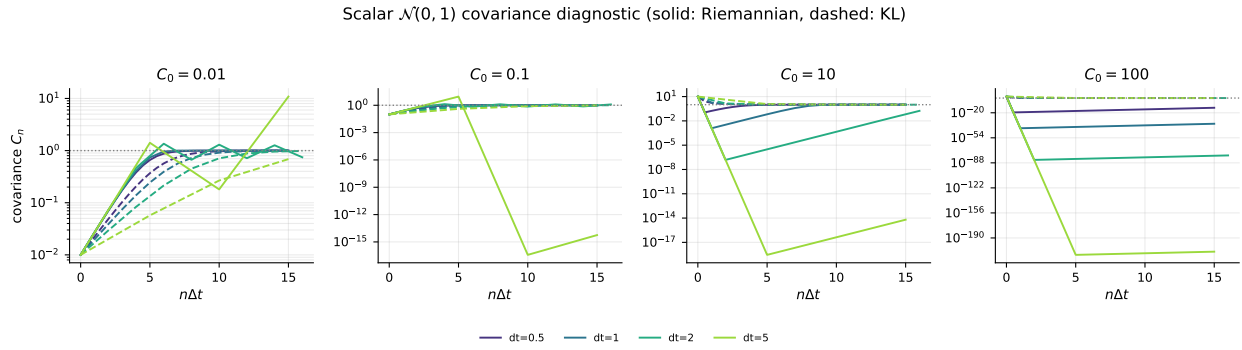
Figure 8: Scalar \mathcal{N}(0, 1) covariance diagnostic. Solid: Riemannian; dashed: KL; color shade encodes \Delta t ; dotted grey: target C = 1 . The KL covariance contracts to 1 for all (C_0, \Delta t) shown.
