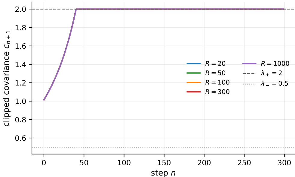
Projected covariance pinned to [\lambda_-, \lambda_+]
