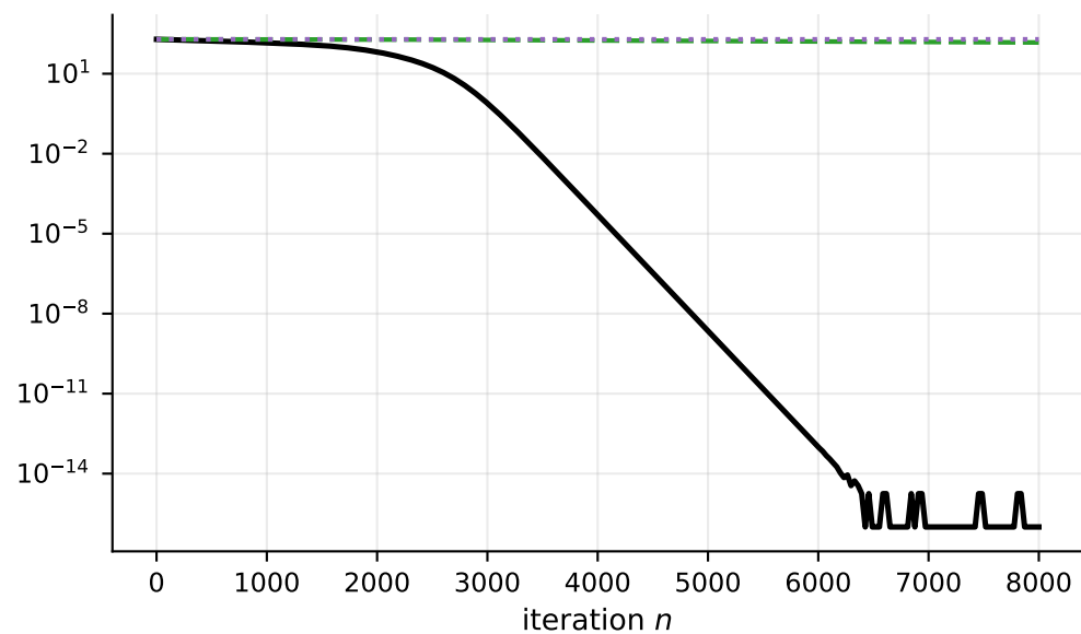
Riemannian, \kappa = 100
