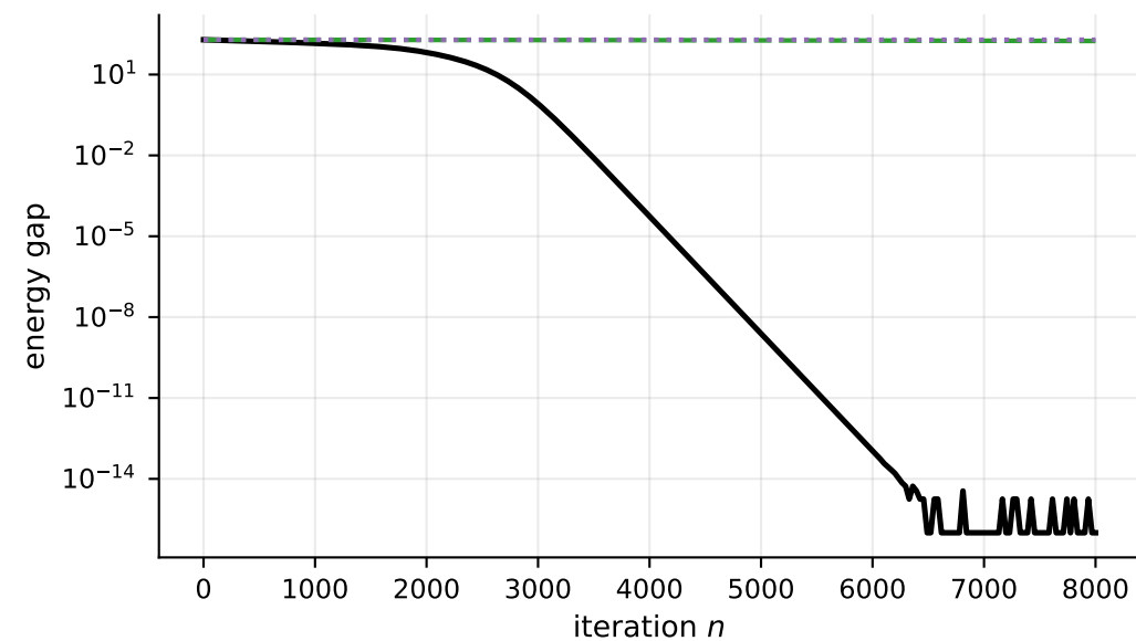
KL, \kappa = 100
