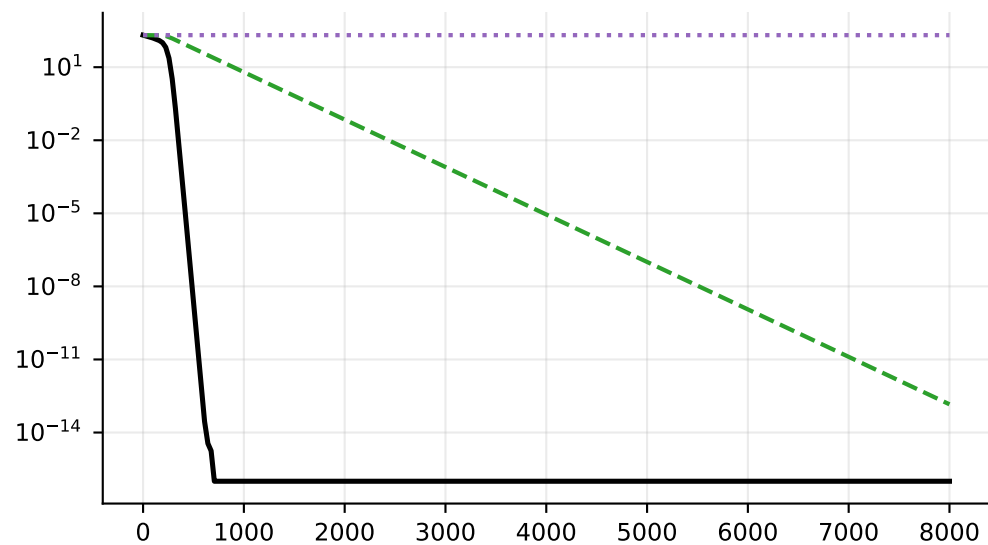
Riemannian, \kappa = 100
