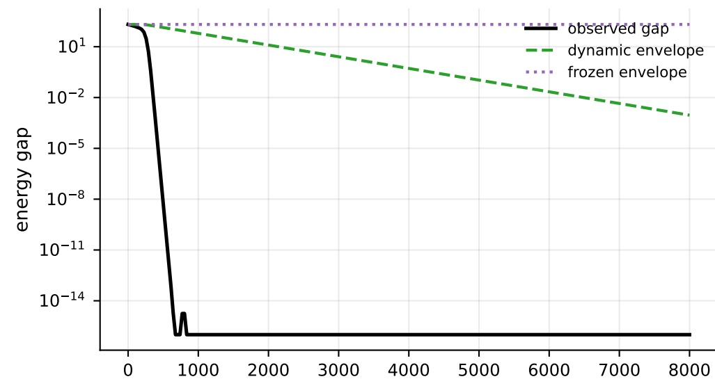
KL, \kappa = 100
