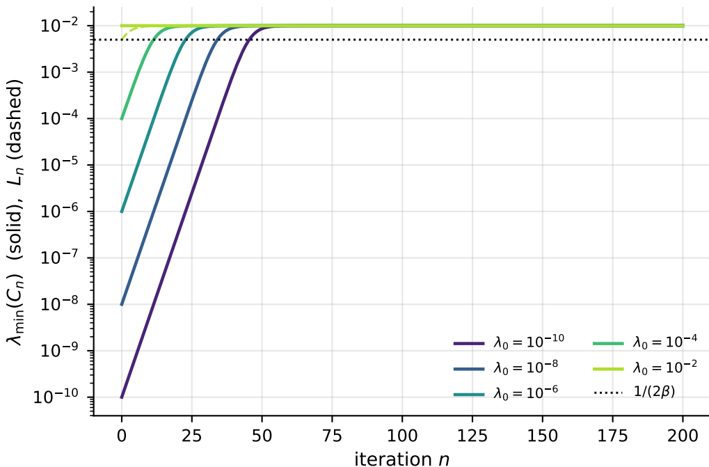
KL covariance envelope ( \kappa = 100, d = 20 )
