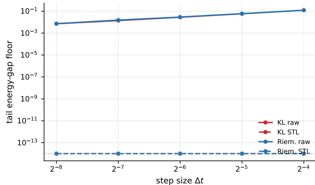
Gaussian ( \Psi_* = 0 )
