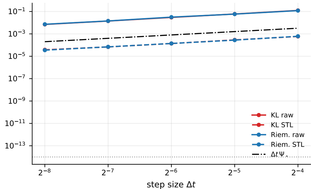
log-cosh ( \Psi_* = 0.051 )
