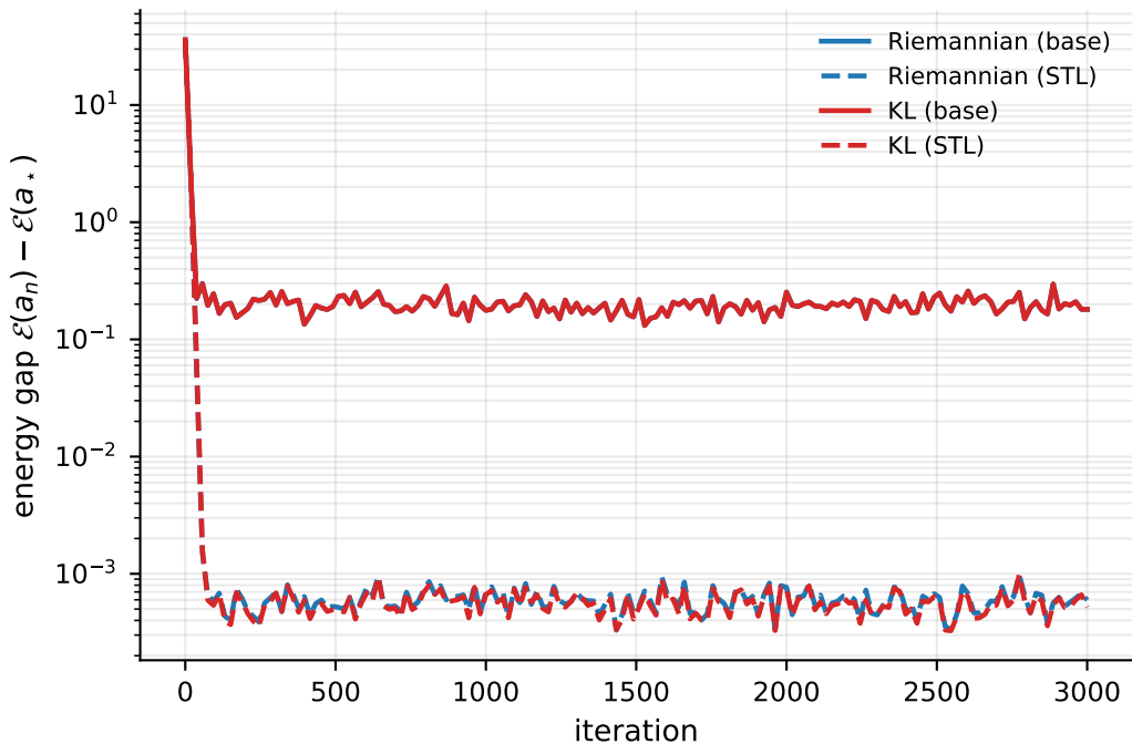
misspecified log-cosh: gap vs iteration ( d = 8, \kappa = 100, \tau = 1, B = 1 )
