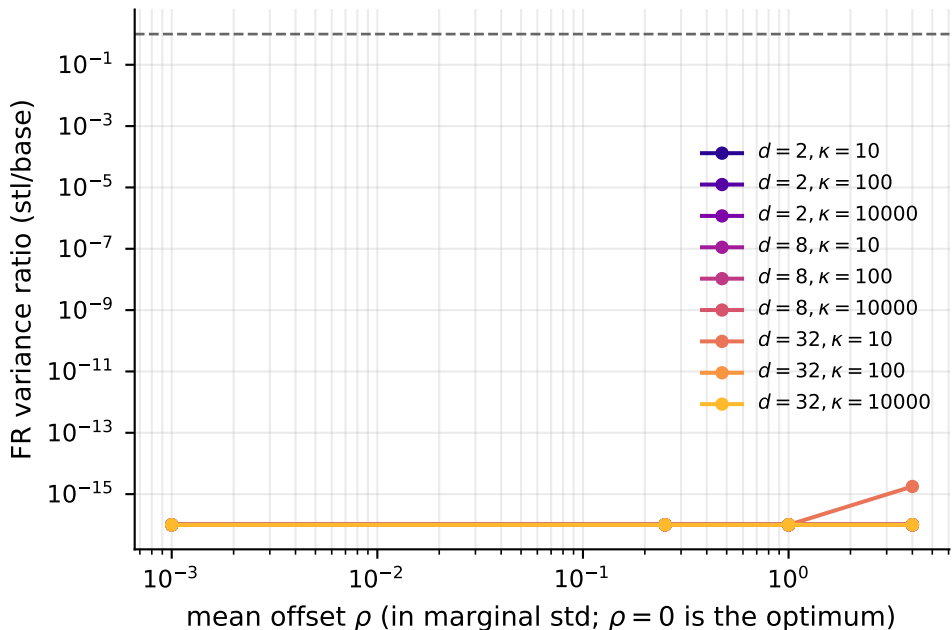
STL variance ratio vs distance -- well-specified Gaussian
