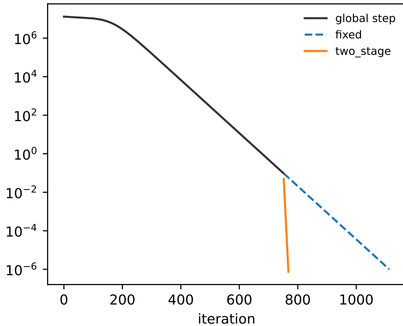
Riemannian
