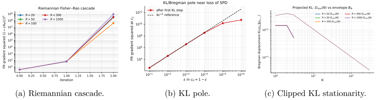
Figure 5: The non-log-concave boundary. Although the Hessian satisfies |V_R''| \leq 1 , negative curvature drives the covariance cascade of Theorem 2.32 and the rational pole of Theorem 2.33 . With the covariance constrained to [\lambda_-, \lambda_+] and a stepsize in the window of Theorem 2.36 , the running minimum of the centered covariance KL stays below the energy-drop envelope. Once the upper constraint binds, the iterate remains pinned and the next displacement vanishes, which is constrained stationarity and not a small unconstrained Fisher–Rao gradient.
