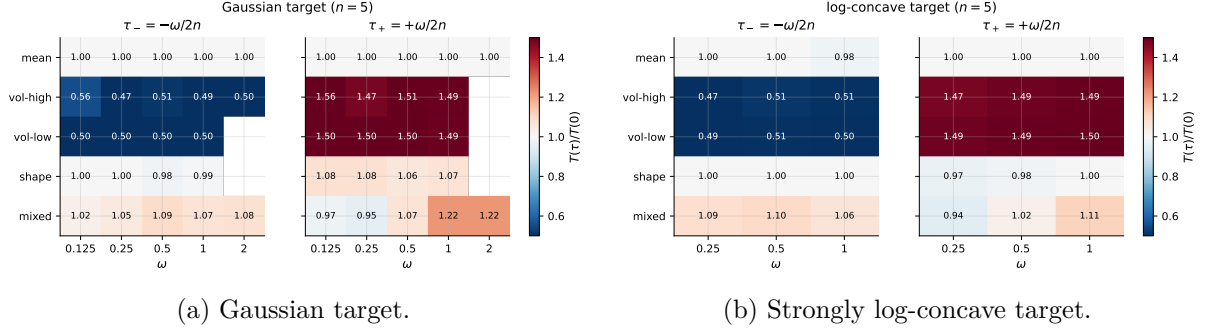
Figure 4: Mode preconditioning in the affine-invariant family. The Gaussian panel calibrates the exact modal computation of Theorem 5.4 ; the non-Gaussian panel is an illustration of the same preconditioning effect and not a convergence theorem for the full metric family, in the sense of Theorem 5.6 .
