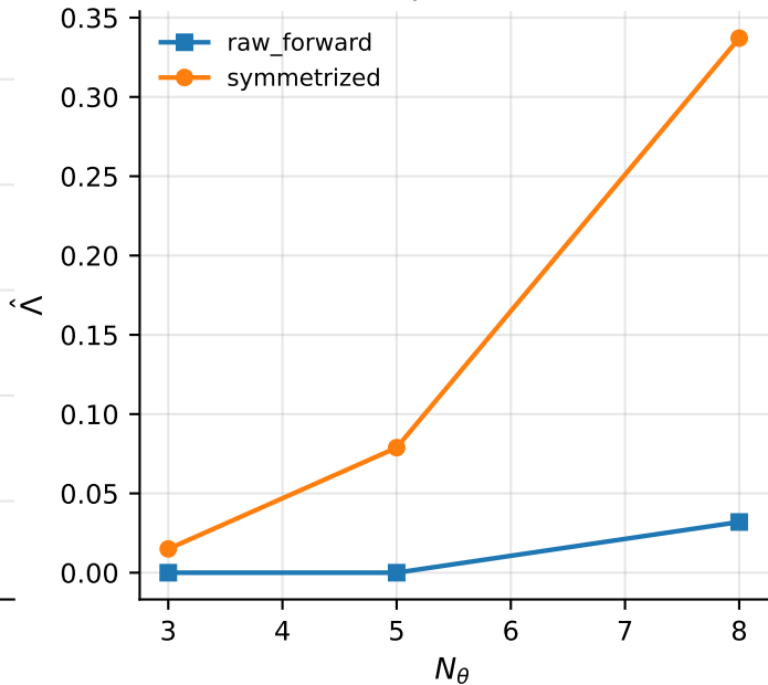
Raw forward vs symmetrized operator norm random_feature separable
