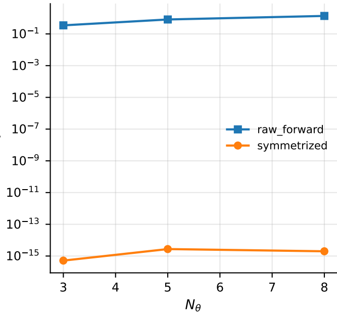
H self-adjointness error: raw forward vs symmetrized random_feature separable
