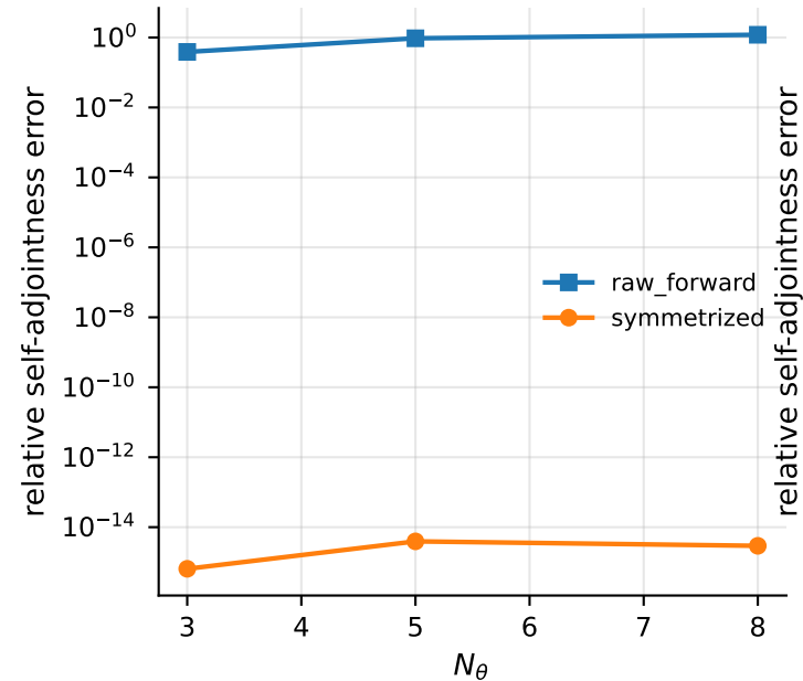
H self-adjointness error: raw forward vs symmetrized random_feature separable
