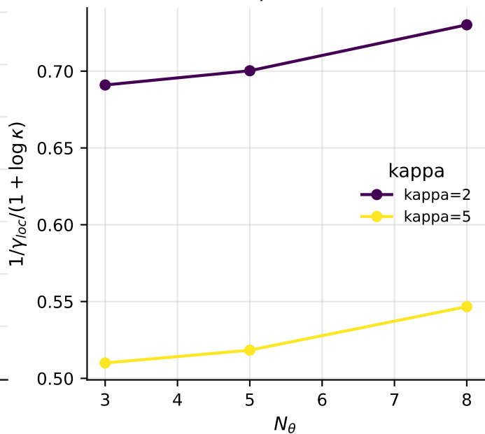
Normalized inverse local rate vs dimension random_feature separable
