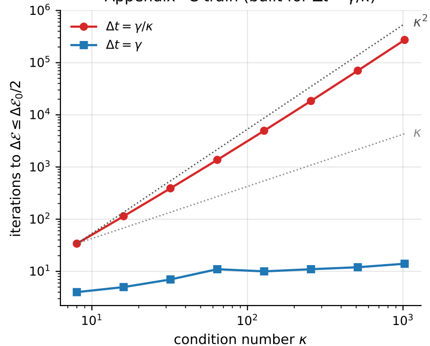
Appendix~C train (built for \Delta t = \gamma/\kappa )
