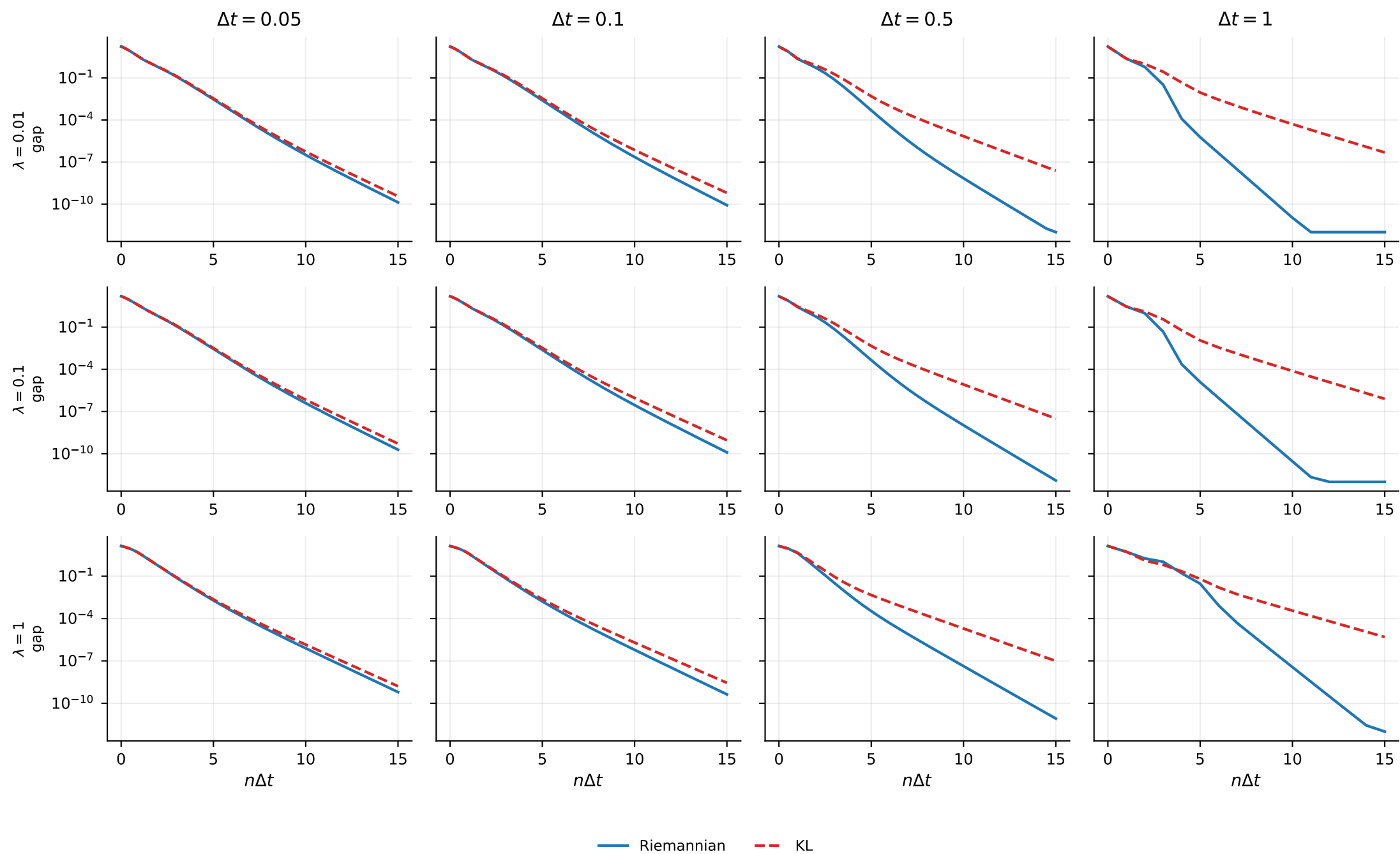
smooth strongly log-concave: convergence at matched stepsize (Riemannian vs KL)
