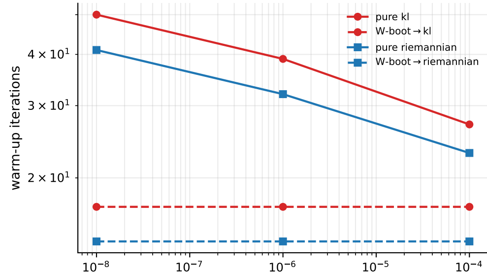
Gaussian: iterations to gap < 10^{-1}
