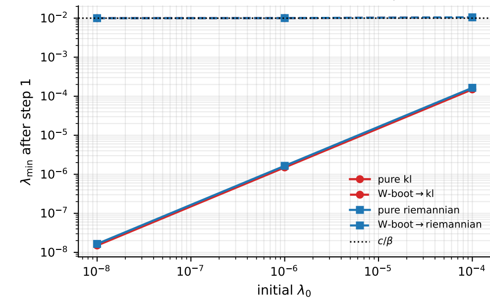
Gaussian: \lambda_{\min}(C) after warm-up
