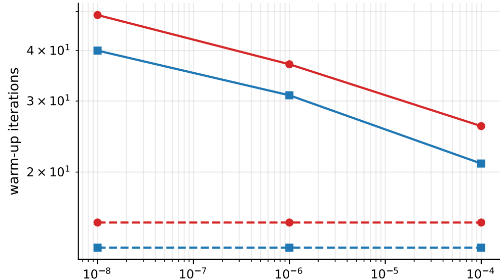
log-cosh: iterations to gap < 10^{-1}
