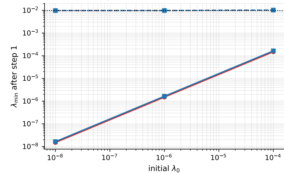
log-cosh: \lambda_{\min}(C) after warm-up
