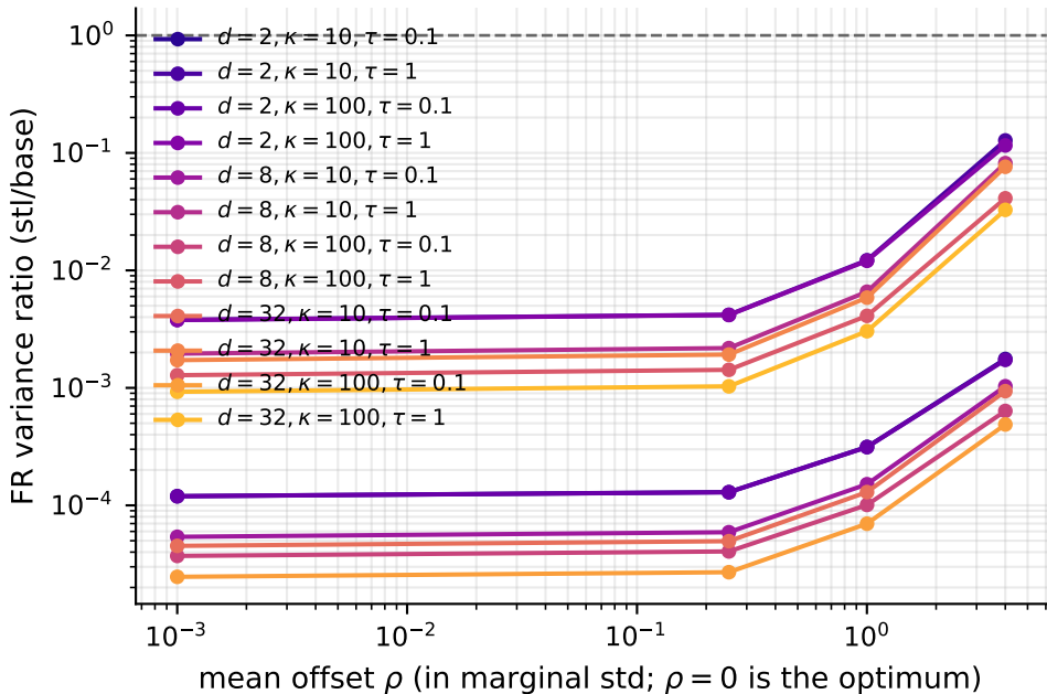
STL variance ratio vs distance -- misspecified log-cosh
