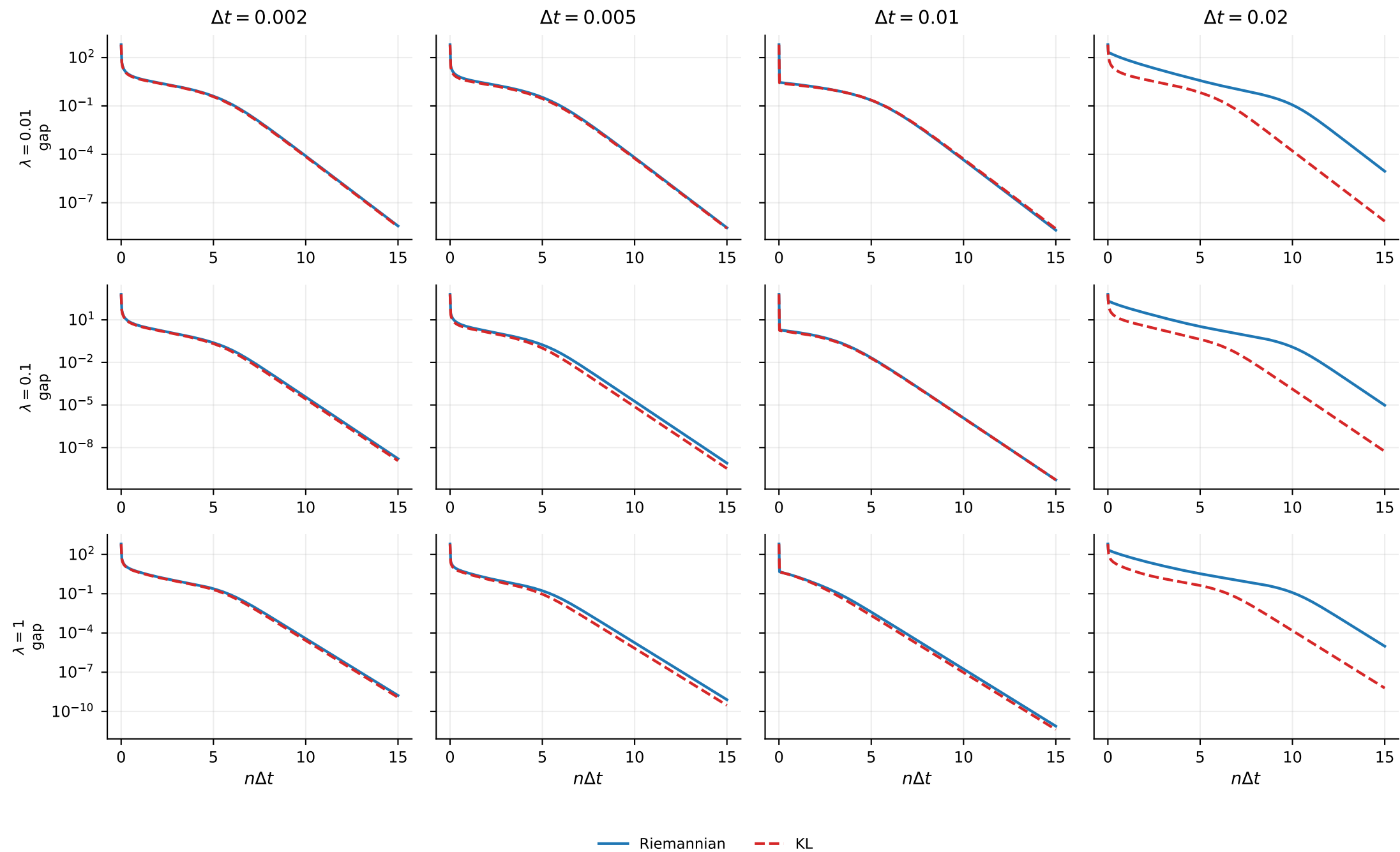
non-smooth log-concave: convergence at matched stepsize (Riemannian vs KL)
