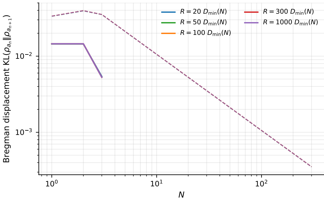
Projected KL: D_{\min}(N) vs envelope B_N
