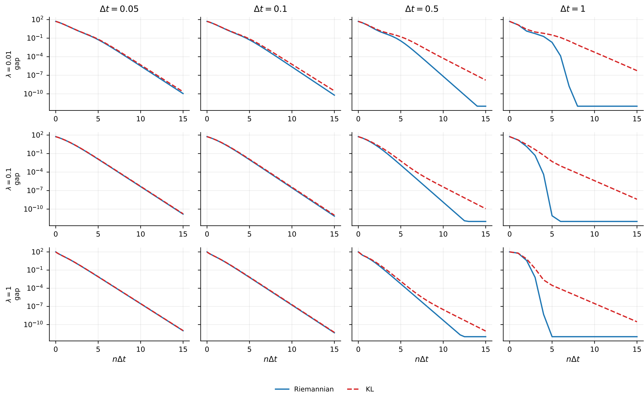
Gaussian posterior: convergence at matched stepsize (Riemannian vs KL)
