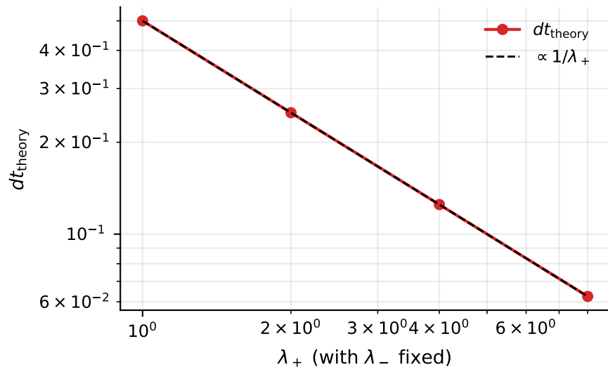
Scales like 1/\lambda_+
