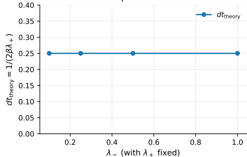
Independent of \lambda_-
