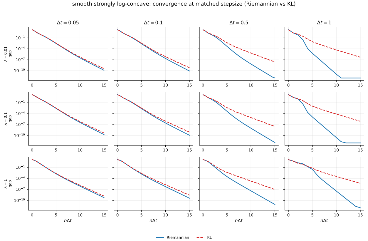
Figure 11: Smooth strongly log-concave posterior: energy gap vs elapsed time n\Delta t (same layout and legend as Fig. 10). The same regime split holds: matched-stepsize agreement at fine \Delta t , and a growing Riemannian advantage as \Delta t coarsens.
