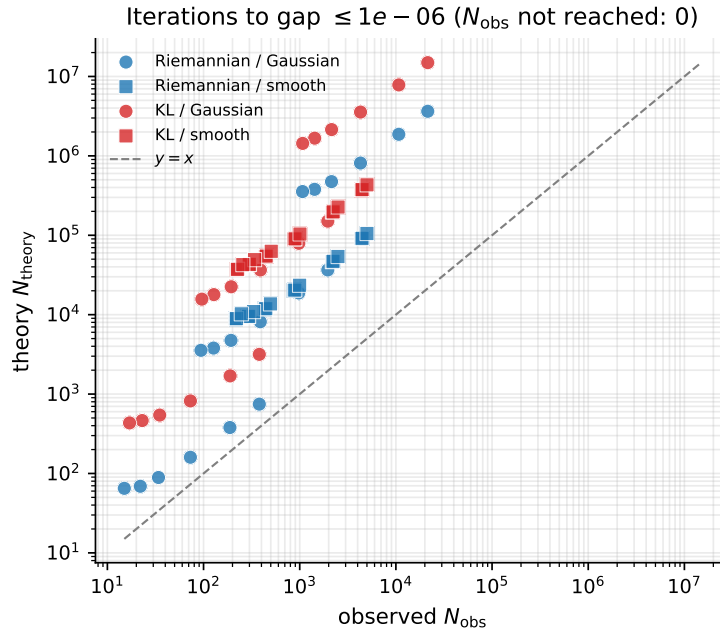
Figure 18: Theoretical vs observed iterations to gap \leq 10^{-6} on the common grid. Points plotted only where both are finite; the count of runs whose observed trajectory does not reach 10^{-6} within T is annotated. Where both are defined, N_{\text{theory}} > N_{\text{obs}} (above y = x ), most strongly for KL.
