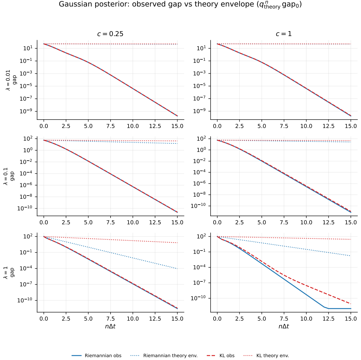
Figure 14: Gaussian posterior: observed energy gap (solid Riemannian, dashed KL) versus the method-specific theory envelopes q_{\text{theory}}^n \text{gap}_0 (dotted), rows \lambda , columns c = \Delta t / \Delta t_{\text{ref}} . Both envelopes sit well above the observed curves; the KL envelope (dotted red) is the higher of the two.
