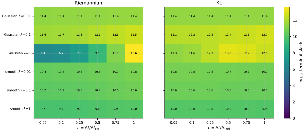
Figure 17: \log_{10} terminal slack q_{\text{theory}}^N \text{gap}_0 / \text{gap}_N per target/ \lambda/c , Riemannian (left) vs KL (right). Larger is more conservative. The slack is large and positive throughout for both schemes; it is largest for KL at the finer fractions, while at the coarsest fractions the Riemannian observed gap reaches near machine precision (deeper observed convergence) and its slack rises into the KL range. A trailing * marks a run whose observed gap reached the numerical floor (slack is then a lower bound).
