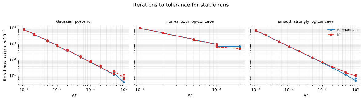
Figure 9: Iterations to reach gap \leq 10^{-4} for stable runs, vs \Delta t (log-log). At matched \Delta t the two schemes are comparable; the meaningful difference is the range of stable \Delta t , not per-step cost.
