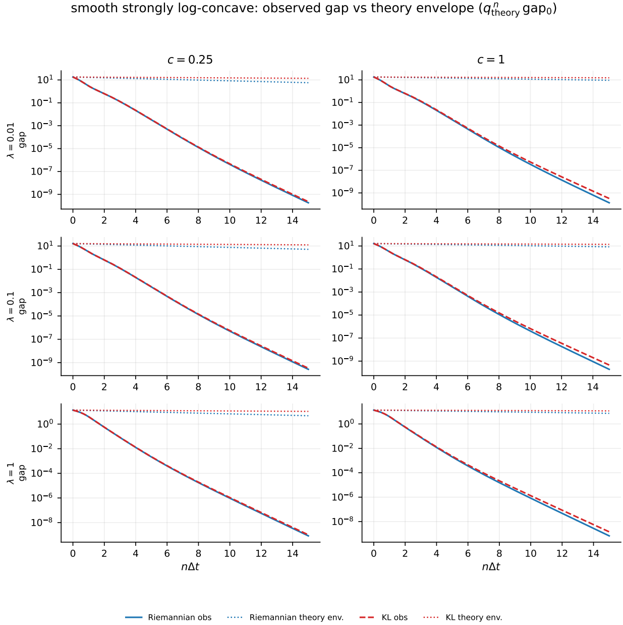
Figure 15: Smooth strongly log-concave posterior: observed gap vs theory envelopes (same layout and legend as Fig. 14). The same ordering holds: observed contraction is faster than both envelopes, with the KL envelope the more conservative.
