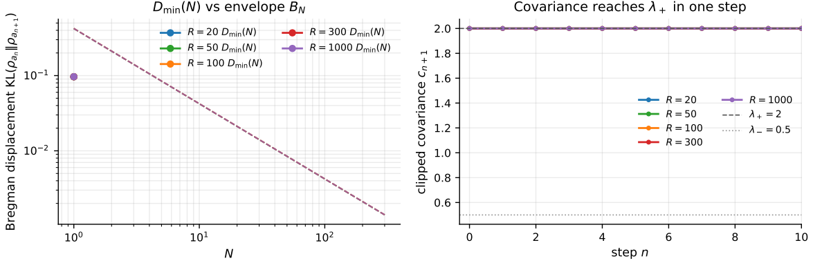
Figure 4: Projected KL at the outside-theorem stepsize \Delta t = 1/(\beta\lambda_+) = 0.5 ( \Delta t L_{\text{clip}} = 2 , twice the theorem edge). Left: the running minimum D_{\min}(N) (markers) versus the envelope B_N (dashed); the only nonzero value is the transient D_0 at N = 1 , below B_1 , after which D_{\min} collapses to zero. Right: the covariance reaches \lambda_+ in a single step and is pinned there.
