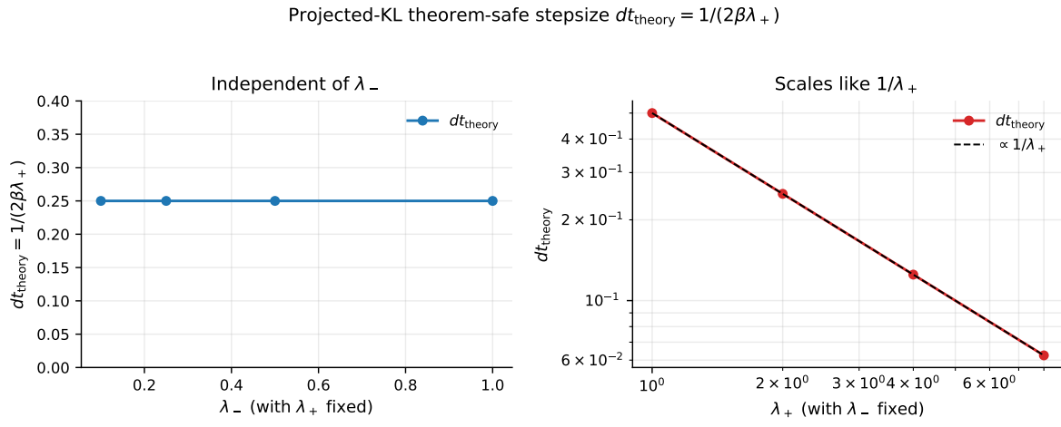
Figure 5: Projected-KL theorem-safe stepsize \Delta t_{\text{theory}} = 1/(2\beta\lambda_+) . Left: varying \lambda_- at fixed \lambda_+ leaves it unchanged. Right: varying \lambda_+ at fixed \lambda_- makes it follow the 1/\lambda_+ reference.
