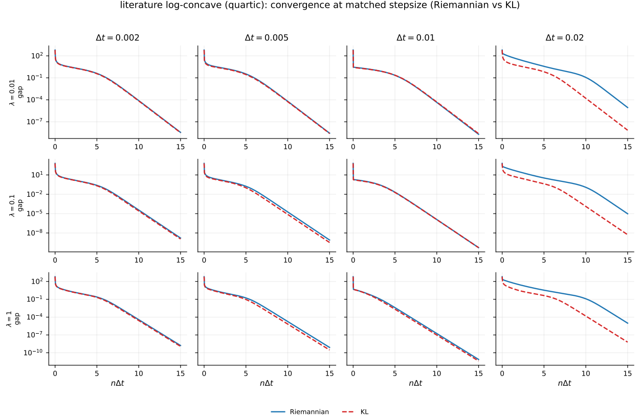
Figure 12: Quartic log-concave posterior: energy gap vs elapsed time n\Delta t (same layout). The convergent stepsizes are an order of magnitude smaller than for the smooth targets; the schemes agree closely at the finer stepsizes, but here KL holds the advantage—most clearly at the coarsest convergent \Delta t = 0.02 , where the Riemannian exponential map sits near its stability edge (terminal gap \sim 10^{-5} ) while KL has converged ( \sim 10^{-9} ). This is the one target on which KL , not Riemannian, is the faster scheme.
