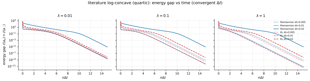
Figure 3: Quartic (non-globally-smooth) log-concave posterior: energy gap vs elapsed time n\Delta t at its convergent representative stepsizes \Delta t \in \{0.005, 0.01, 0.02\} . Both schemes converge cleanly here; the stepsizes are an order of magnitude smaller than for the smooth targets, reflecting the unbounded curvature of the quartic tail. (Larger stepsizes diverge for both methods and are excluded; see the stability heatmap, Fig. 6.)
