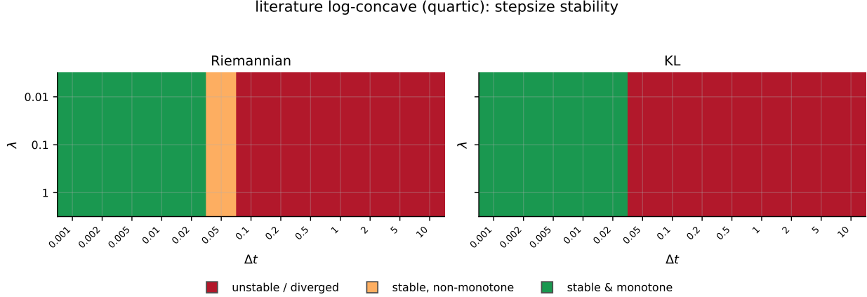
Figure 6: Quartic log-concave stability classification (no theory line, since the target is not globally smooth). Both schemes are stable only for small \Delta t .
