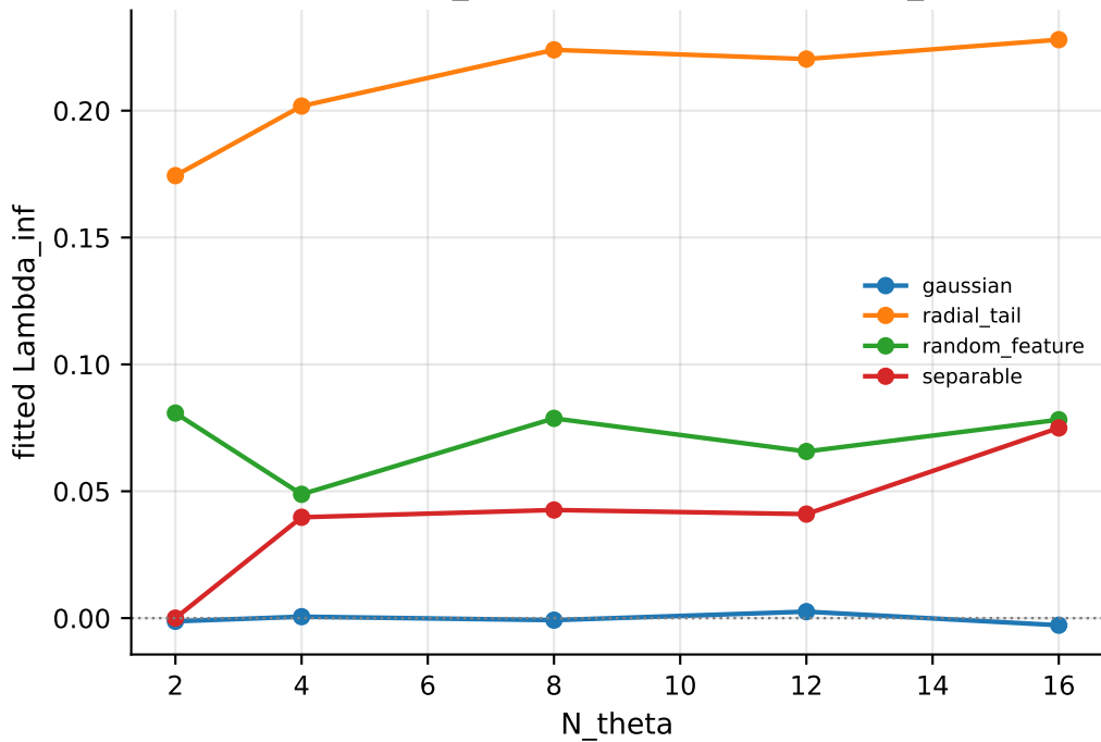
Convergence fit: \text{Lambda\_inf from Lambda} = \text{Lambda\_inf} + c \sqrt{p/M}
