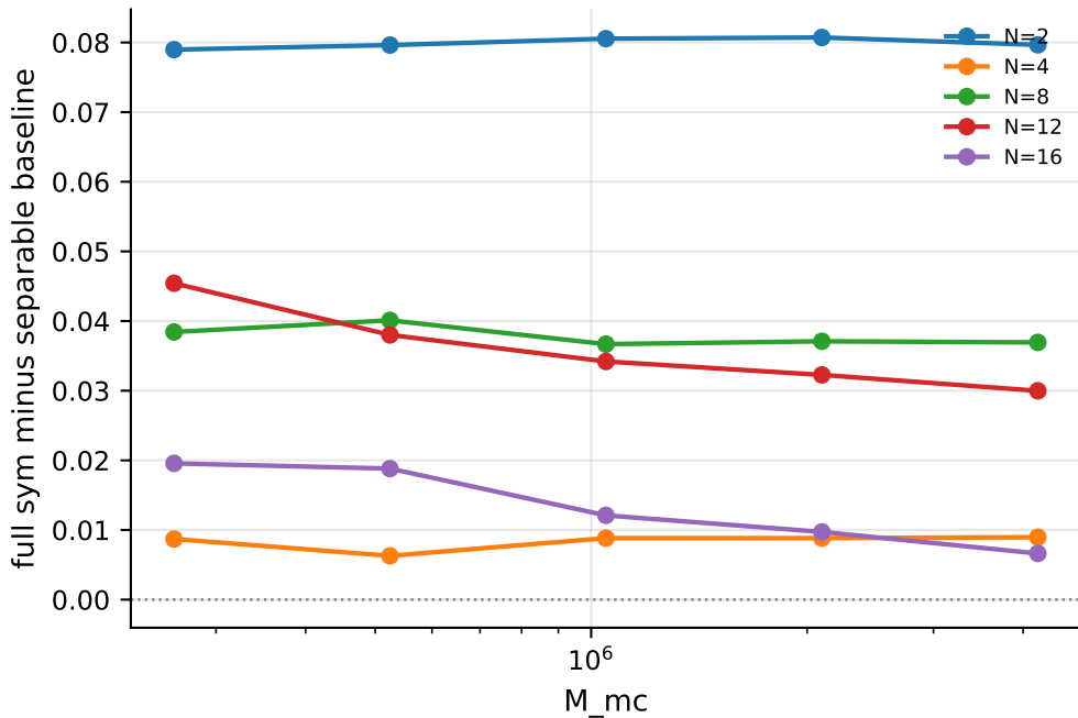
Random feature excess over separable baseline
