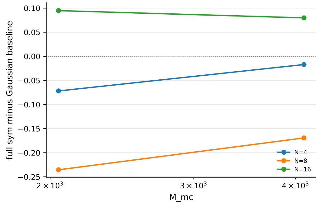
Random feature excess over Gaussian baseline
