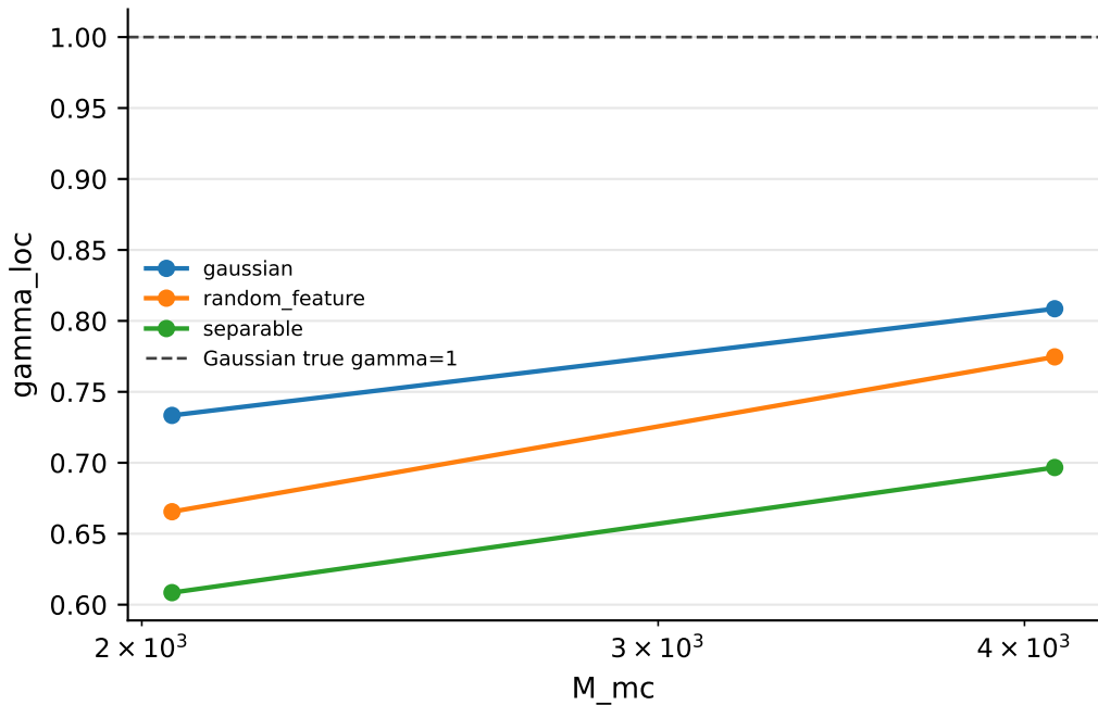
Local rate vs sample size
