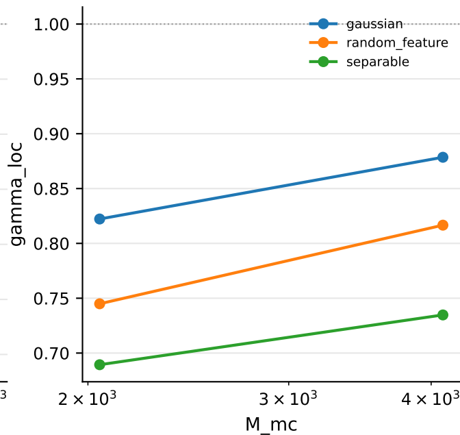
gamma_loc comparison across baselines and potentials
