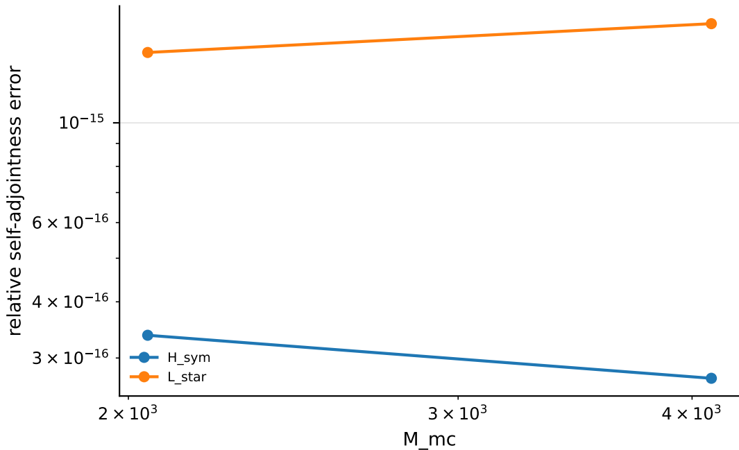
Self-adjointness checks vs sample size
