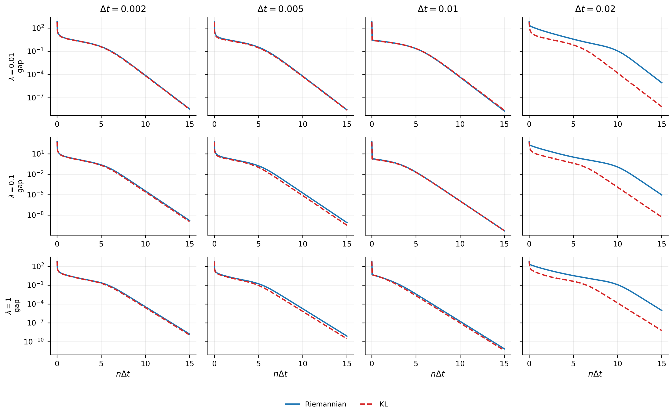
literature log-concave (quartic): convergence at matched stepsize (Riemannian vs KL)
