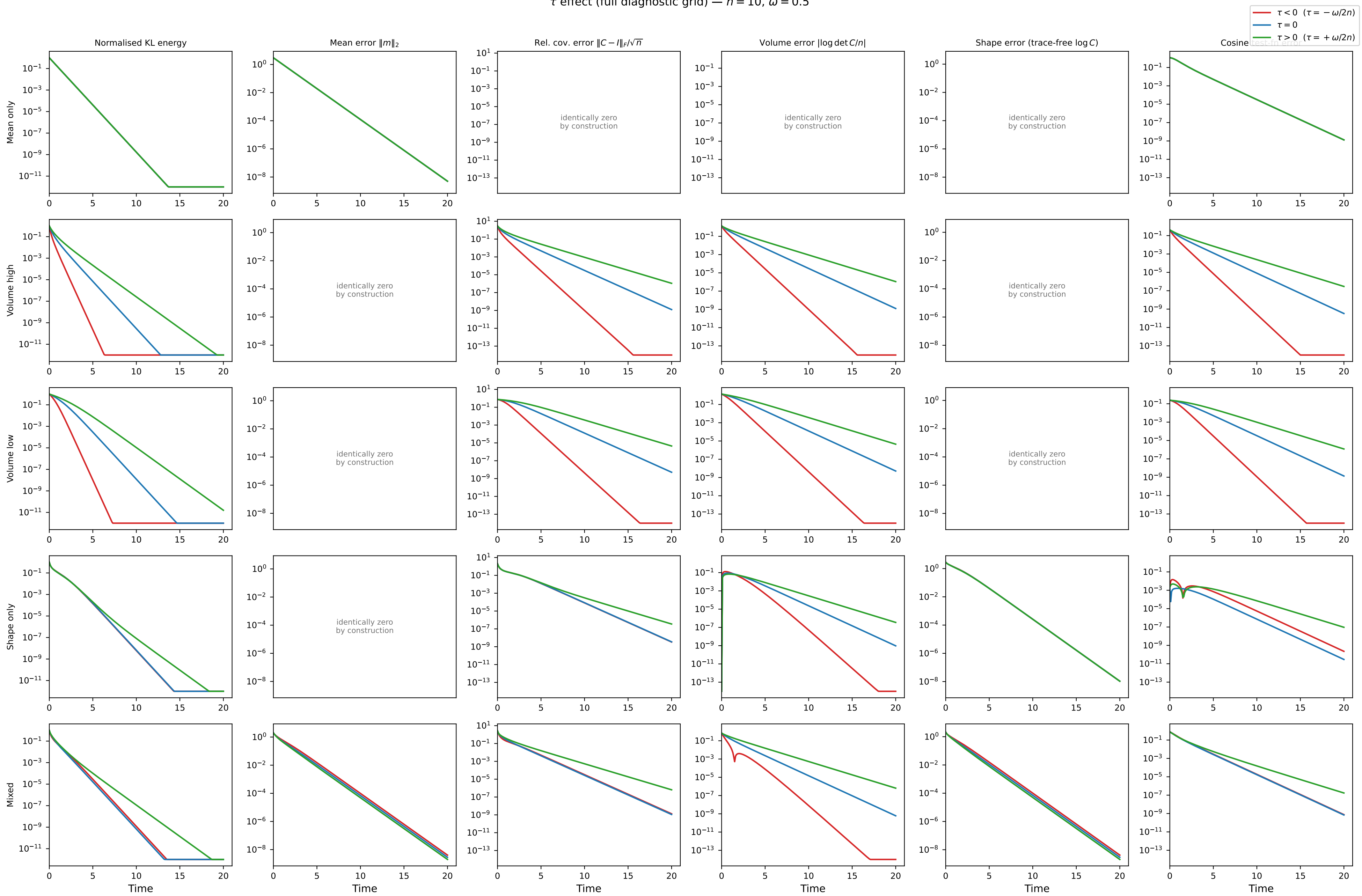
\tau effect (full diagnostic grid) — n = 10, \omega = 0.5
