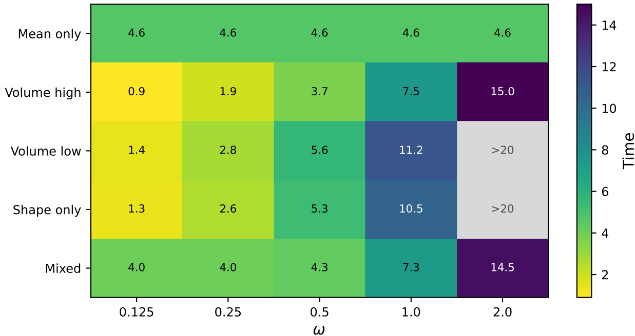
Time to E/E_0 \leq 10^{-4} — n = 5 , \tau = 0
