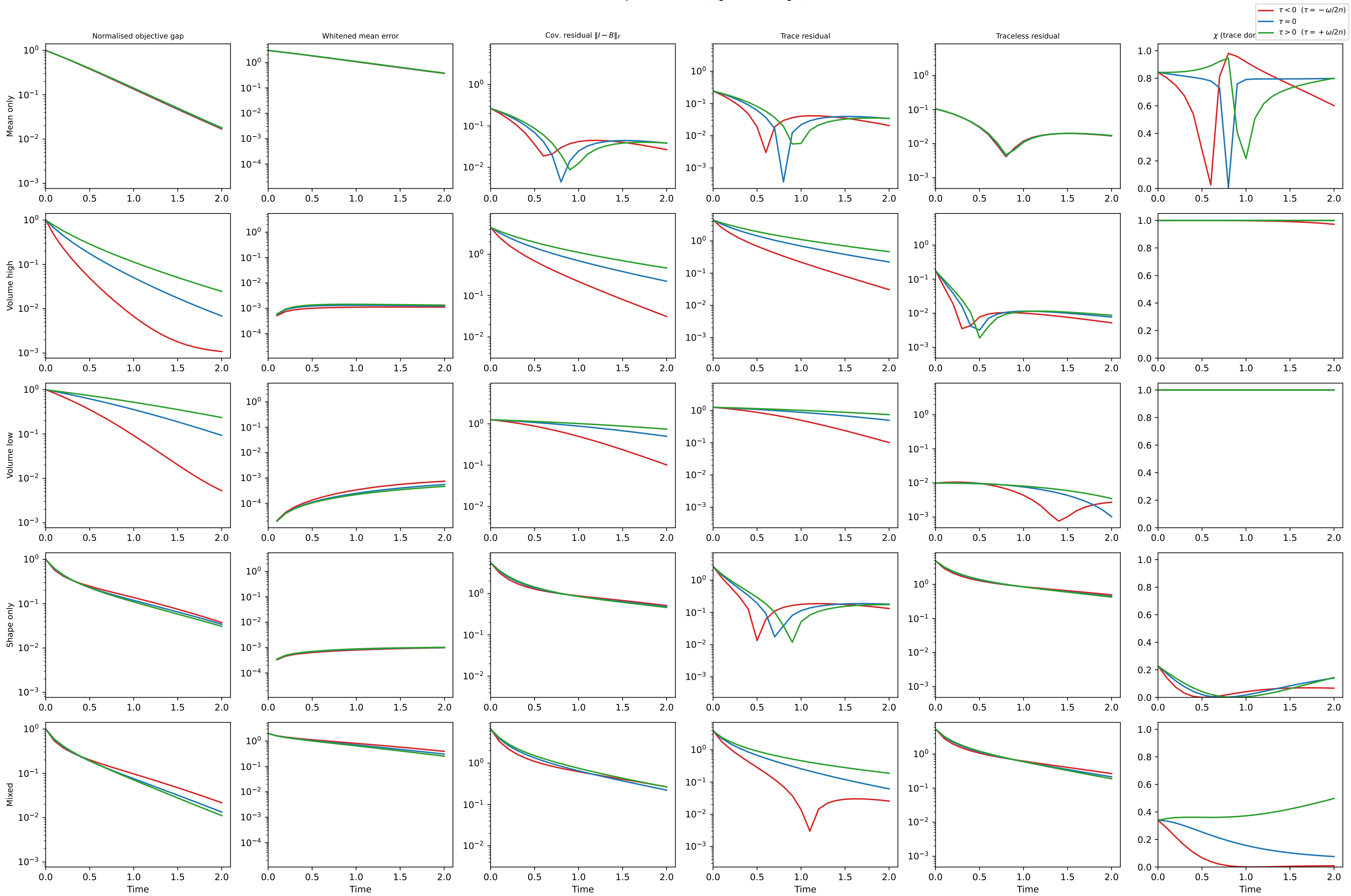
\tau effect — n = 3 , \rho = 2.0 , \omega = 0.5 (log-concave target)
