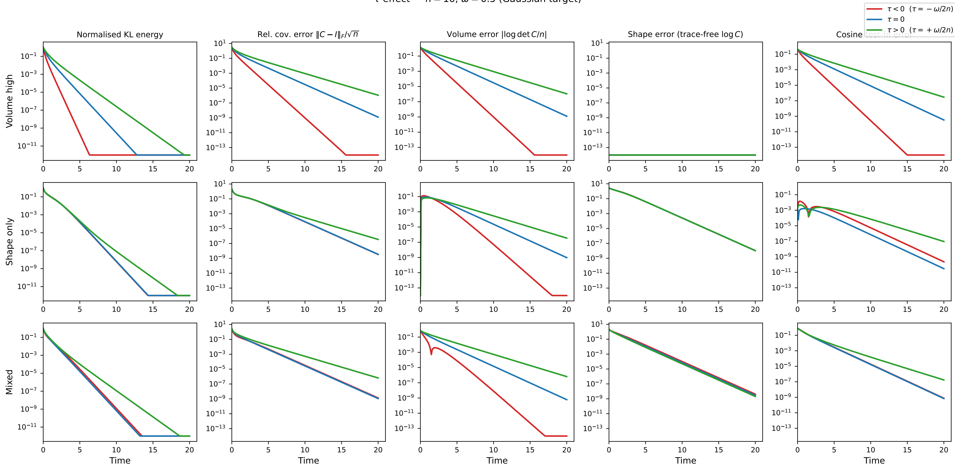
\tau effect — n = 10, \omega = 0.5 (Gaussian target)
