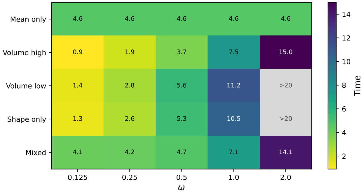
Time to E/E_0 \leq 10^{-4} — n = 2 , \tau = 0
