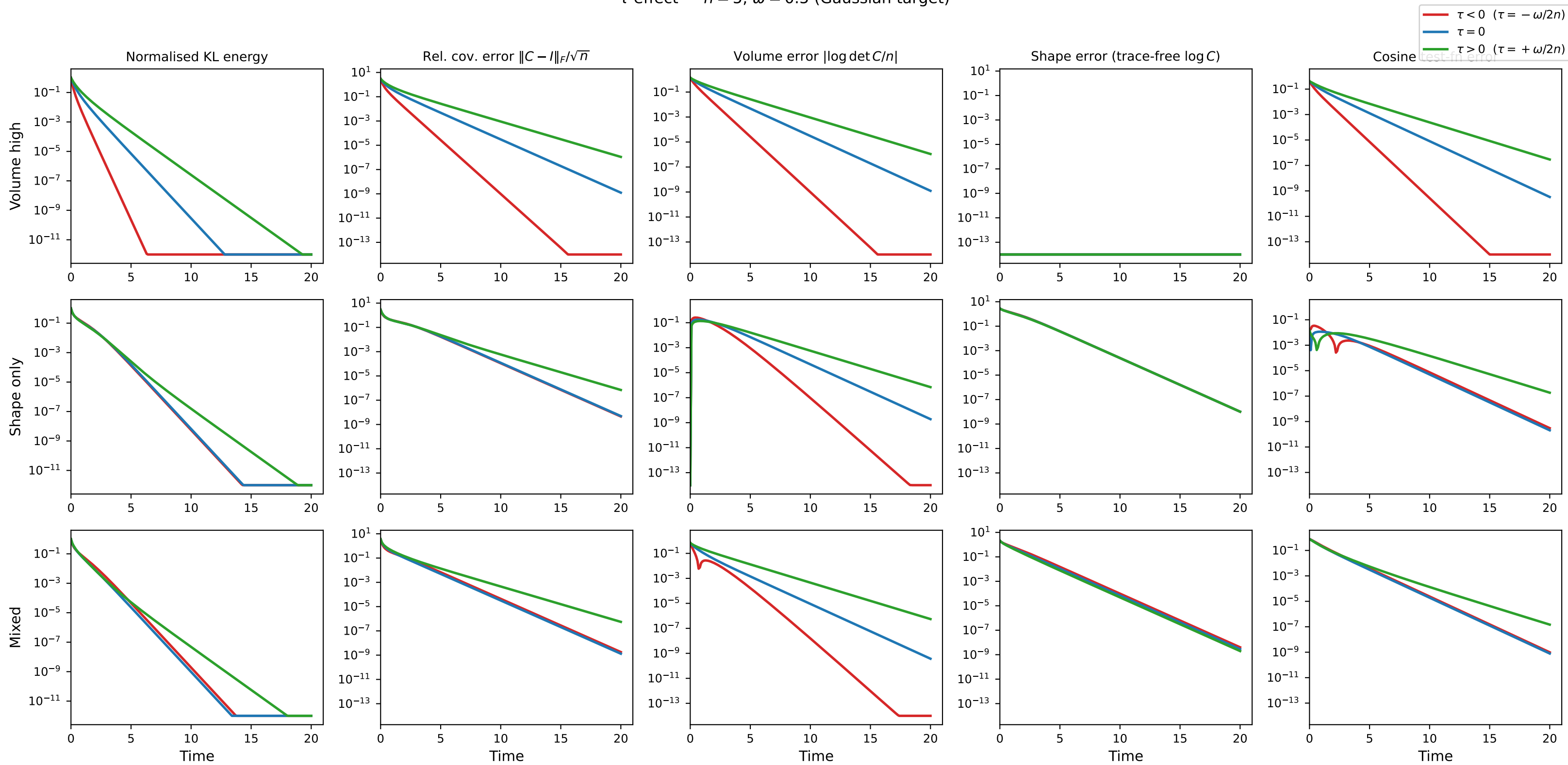
\tau effect — n = 5 , \omega = 0.5 (Gaussian target)
