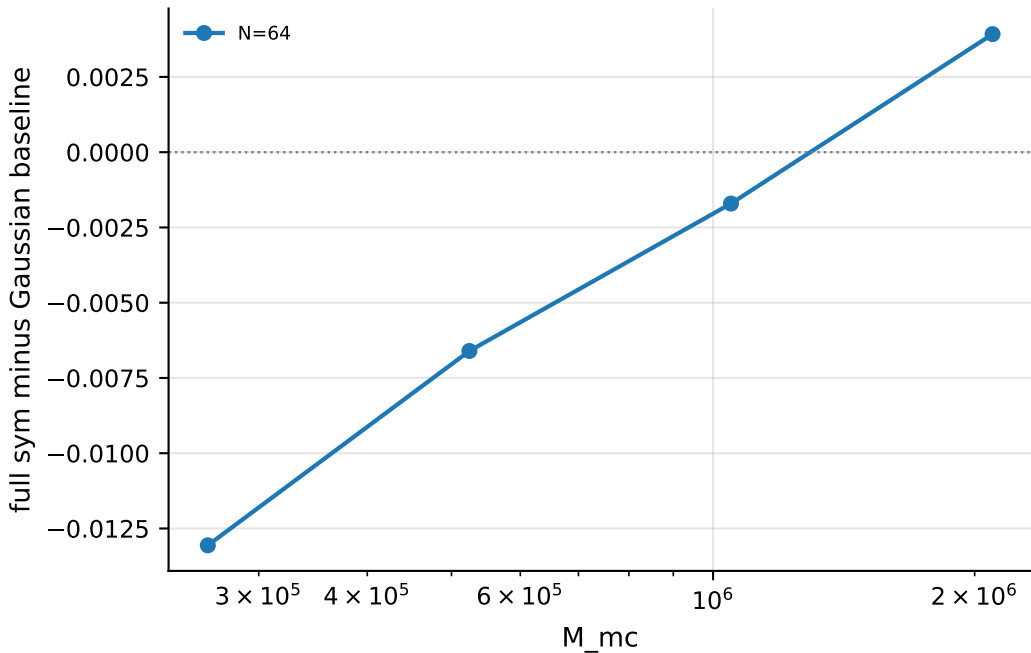
Random feature excess over Gaussian baseline
