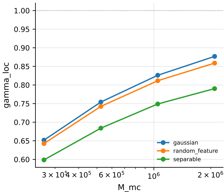
gamma_loc comparison across baselines and potentials N=64
