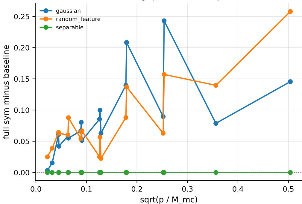
Baseline-corrected gap vs finite-sample noise scale
