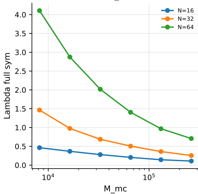
Full operator estimates vs sample size (finite-sample diagnostic)
