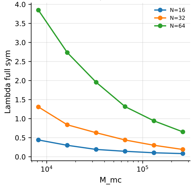
Full operator estimates vs sample size (finite-sample diagnostic)
