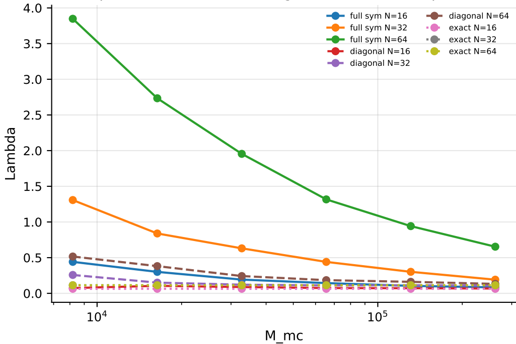
Separable controls: full, diagonal, exact vs sample size
