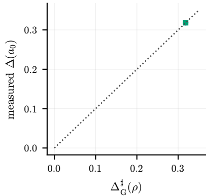
(c) Sharp threshold
