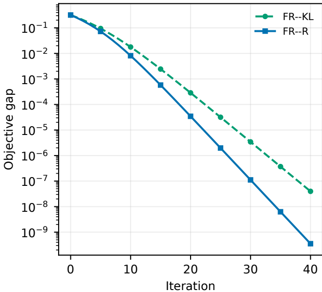
Experiment F
