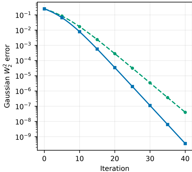
Experiment F
