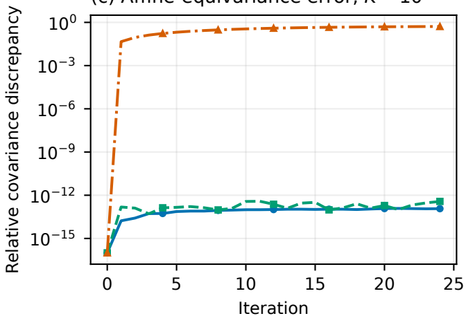
(c) Affine-equivariance error, K = 10^4
